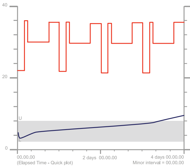
ISTA 7D Hot +2°C to +8°C for 84:10hrs+
