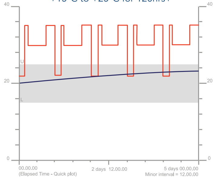
ISTA 7D Hot +15°C to +25°C for 120hrs+
